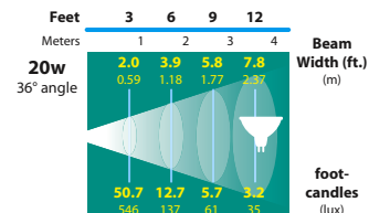
20w MR16 FL (BAB) SL-34-MR16
