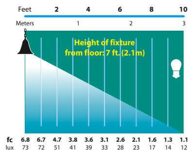
SL-05 Half Spread Photometrics 20 ft. (6.0m) diameter
