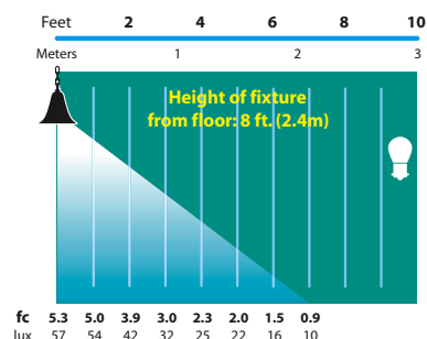
SL-05 Half Spread Photometrics 14 ft. (4.3m) diameter
