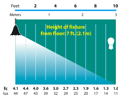
SL-06 Half Spread Photometrics 20 ft. (6.0m) diameter
