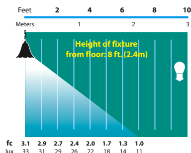
SL-06 Half Spread Photometrics 14 ft. (4.3m) diameter
